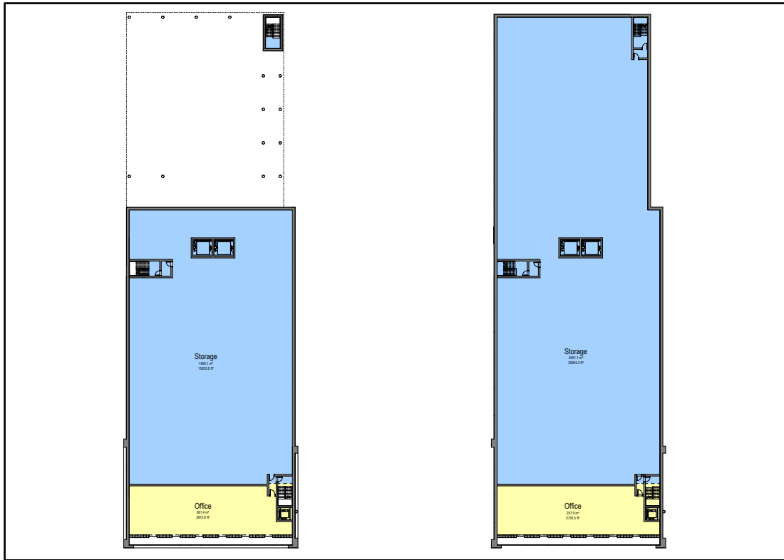
Proposed 1 st and 2 nd Floor Plans
